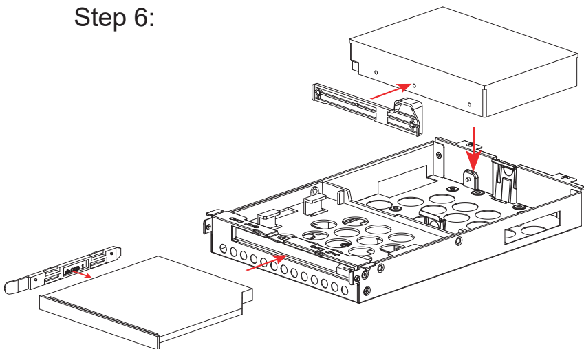
Slim ODD & 3.5 inch HDD
